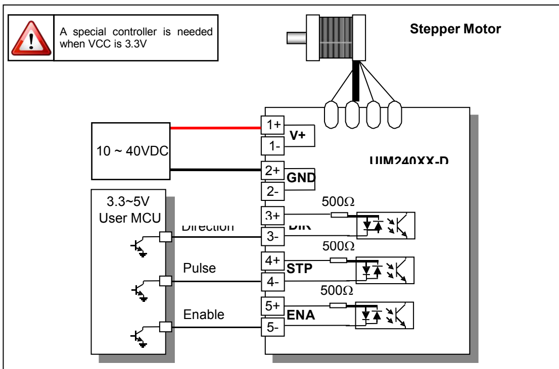
Figure 0-3: Typical Application of UIM240XX-D
