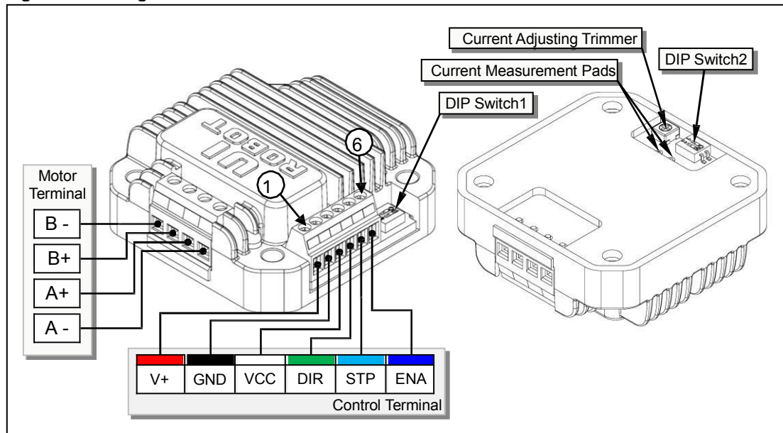
Figure 0-1: Wiring Terminal
